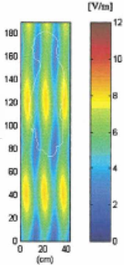
E_{rms} no subject present
