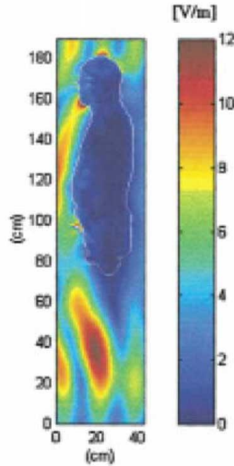
E_{rms} with subject present
